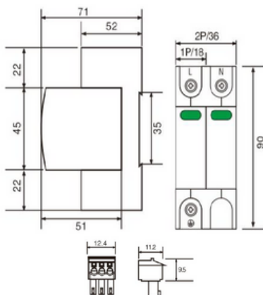
Dimension Drawing (mm)
